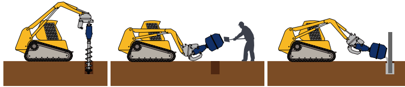
Drill Mix Fill with Skidsteer Loader
